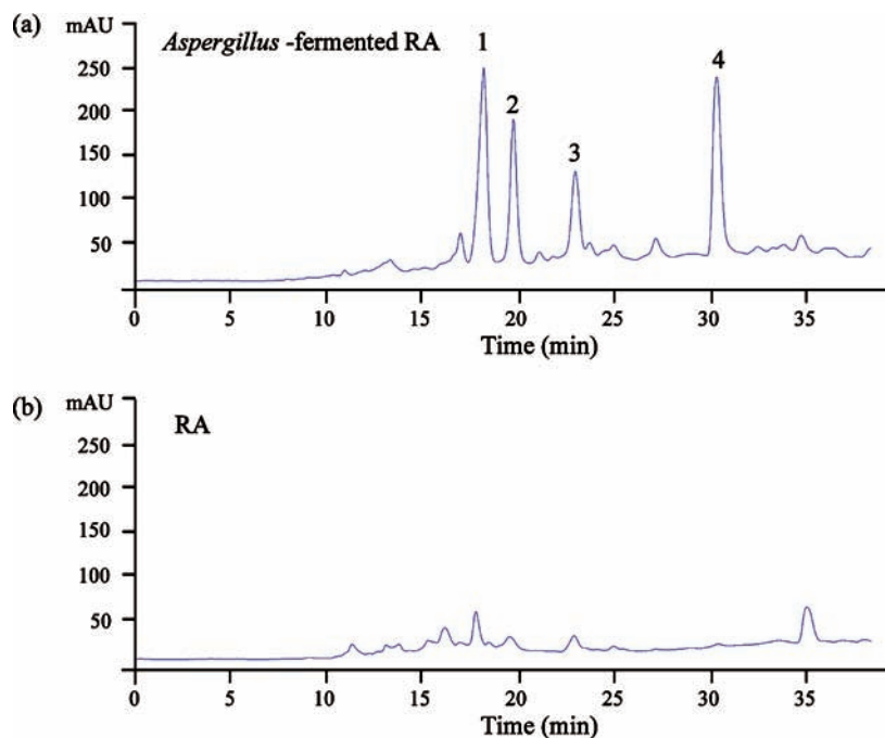
Figure 3. HPLC patterns of RA fermented with A. oryzae M29 (a) and RA without fermentation (b), on an ODS C18 reverse-phase column ( 10 \times 250 mm) eluted with a linear gradient of acetonitrile (5–70% at 0–30 min and 70–85% at 30–45 min) containing 0.1% TFA at 1 mL/min and the pattern detected at 280 nm.
